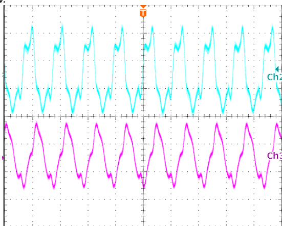
Output voltage ripple at nominal input voltage and max load current Top trace +15V, 10mV/div, Bottom trace -15V, 20mV/div, 2 \mu s/div. Load cap: 10 \mu F, tantalum capacitor and 1 \mu F ceramic capacitor. Bandwidth: 20MHz.
